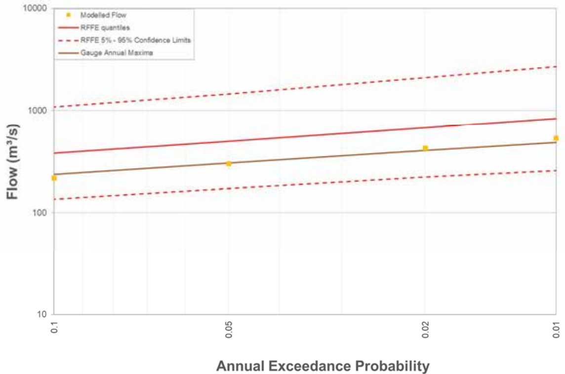
■ Figure 5-1 Verification results compared to the Campaspe River @ Redesdale gauge (406213) and the RFFE
