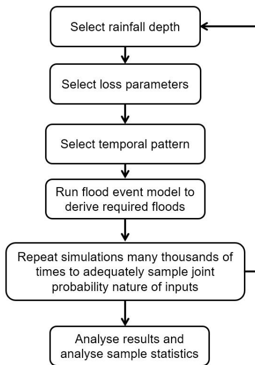
■ Figure 4-3 Overview of adopted joint probability framework
