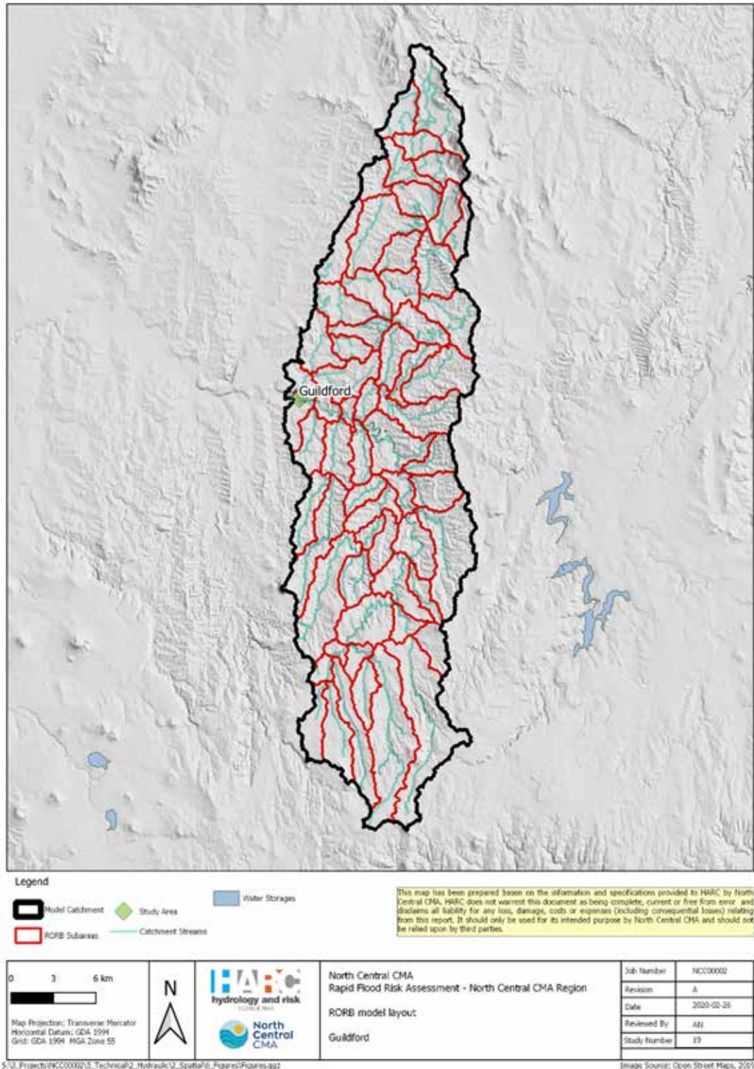
■ Figure 3-1 RORB model layout
