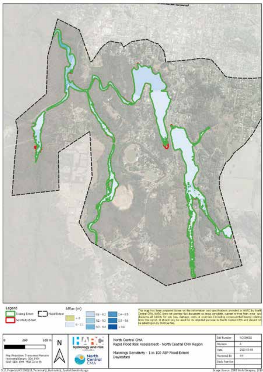
■ Figure 8-5 Manning's n sensitivity analysis result
