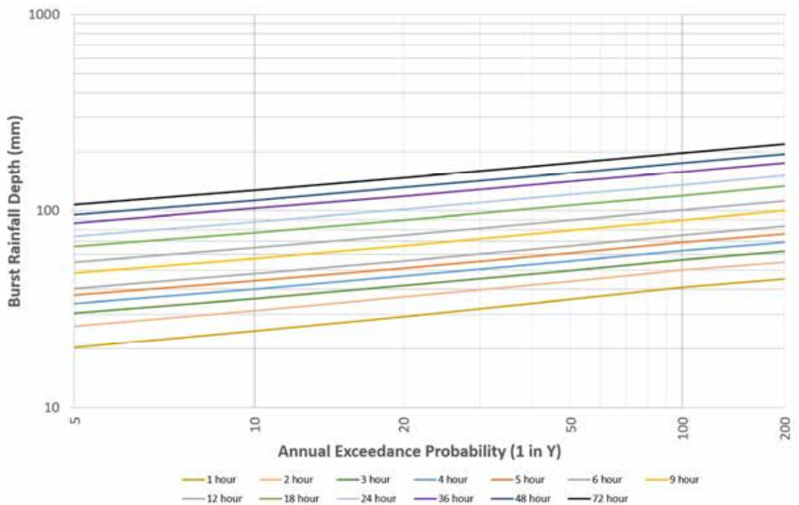
■ Figure 4-4 Adopted design rainfall depths
