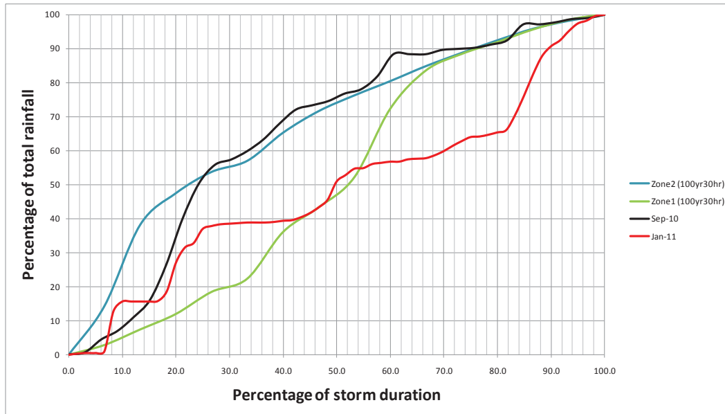
Figure 4-14 Design and observed temporal pattern comparison
