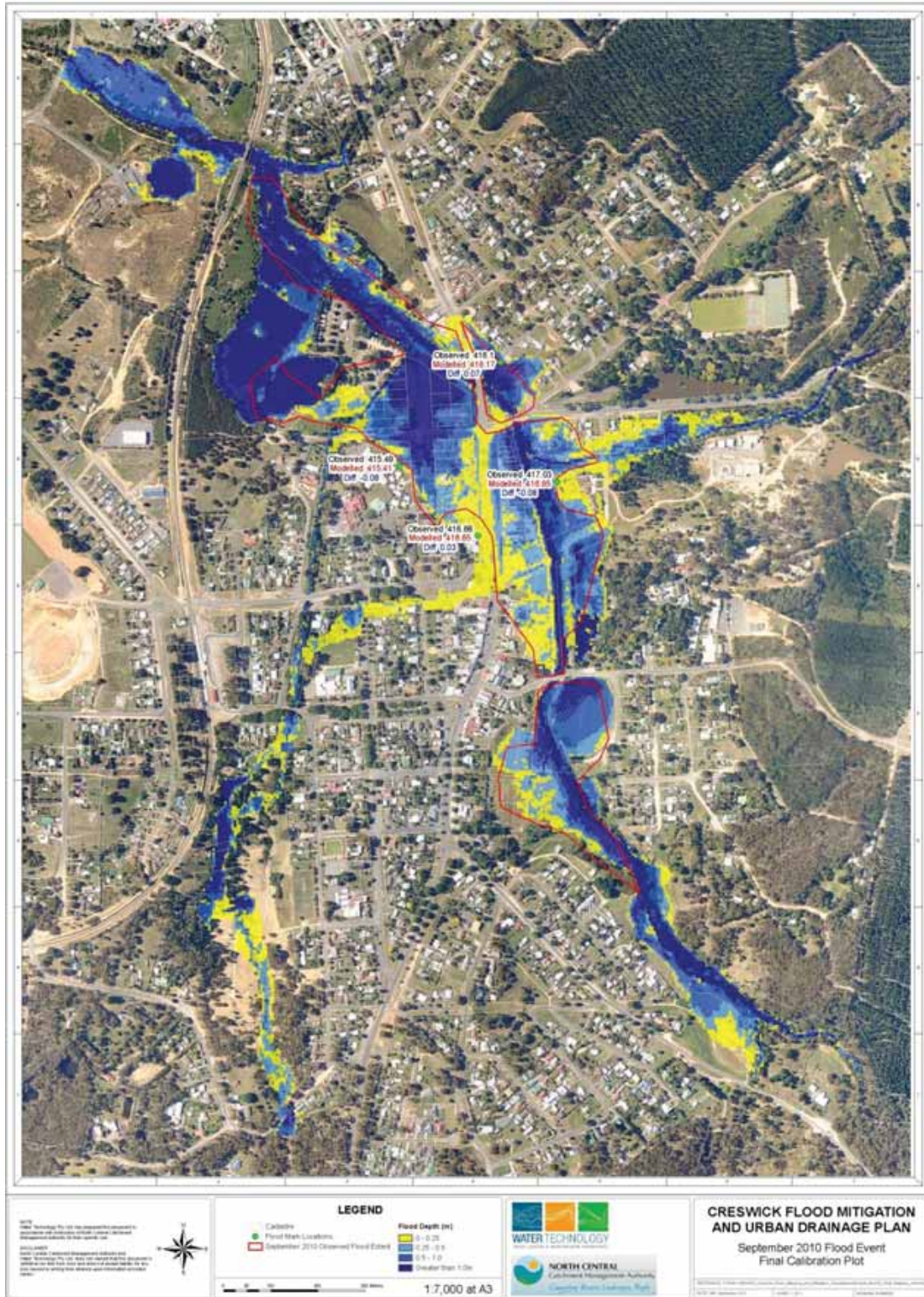
Figure 5-3 Hydraulic model calibration plot – September 2010
