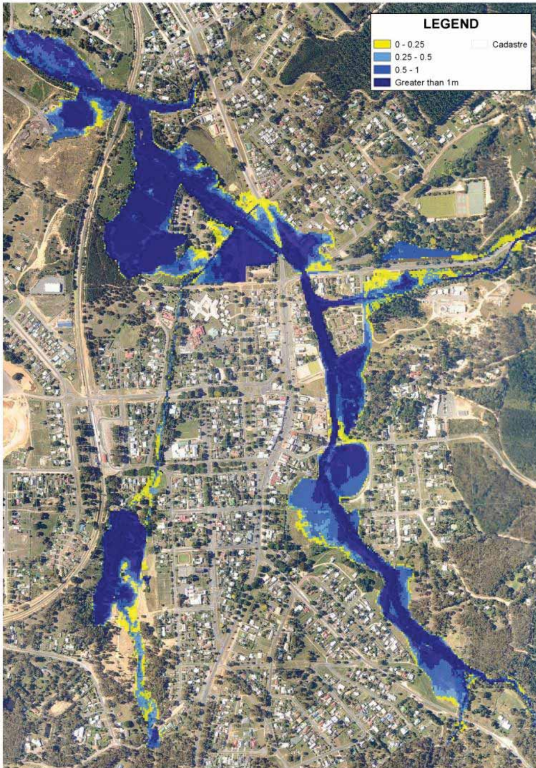
Figure 6-2 Proposed structural mitigation option 1 – 100 year ARI extent
