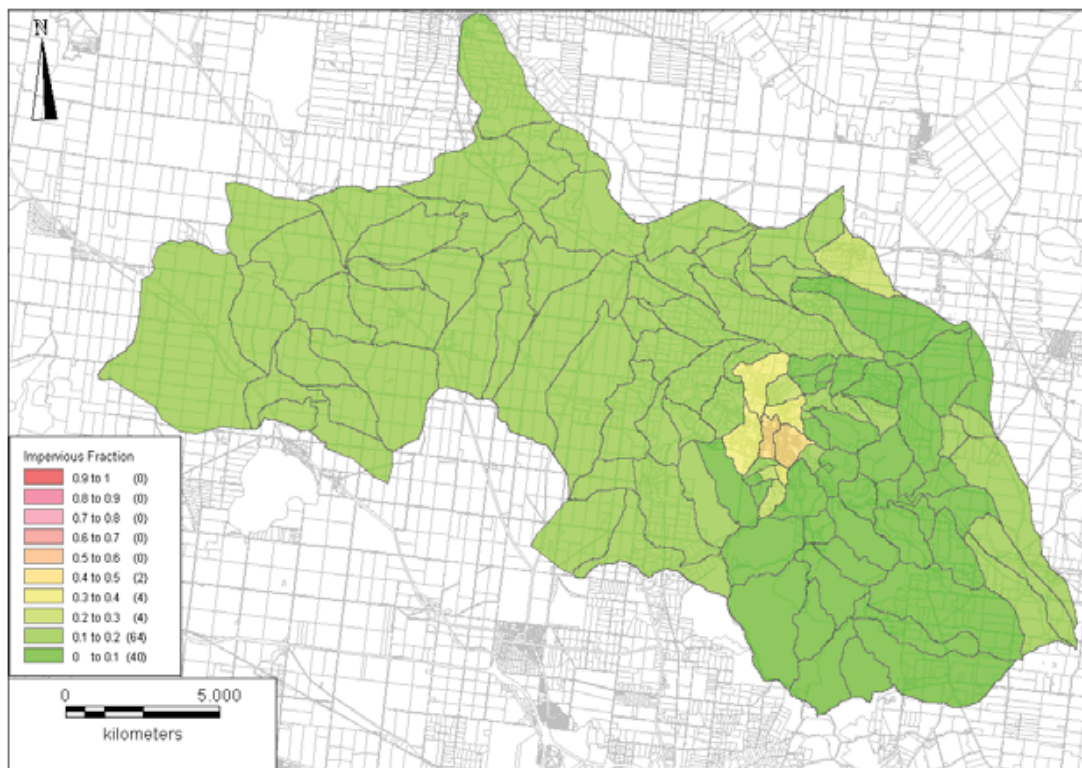
Figure 4-3 RORB model fraction impervious values
