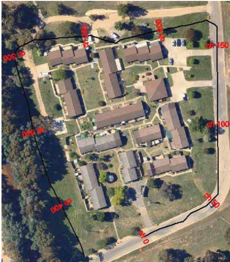
Figure D-2 Semmens Village Levee Alignment
