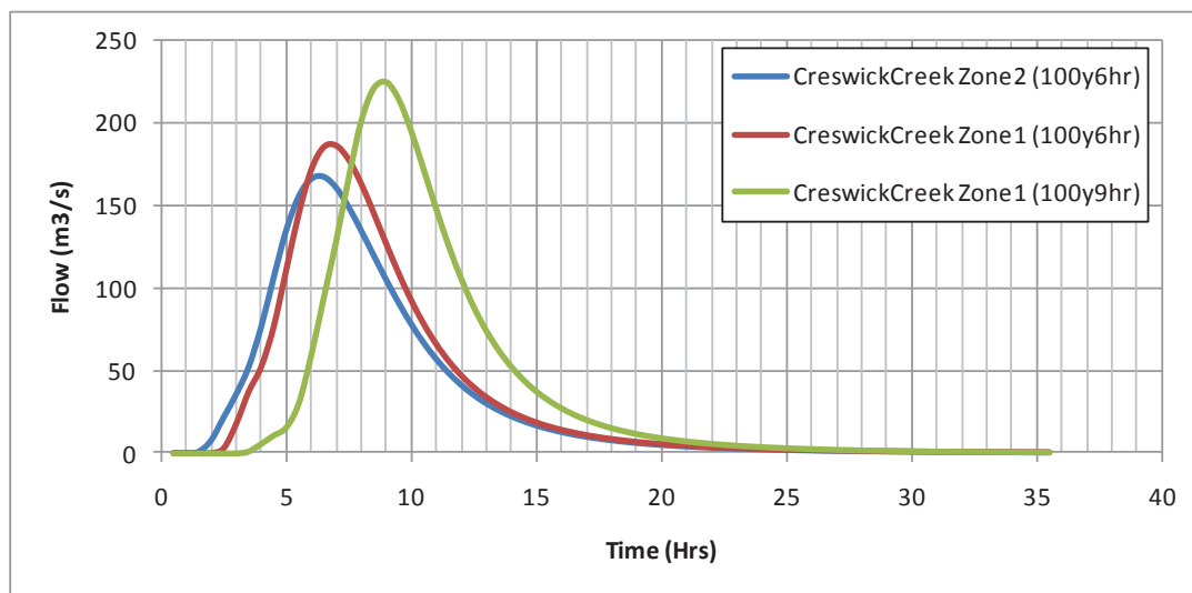
Figure 4-15 Temporal pattern hydrograph comparison
