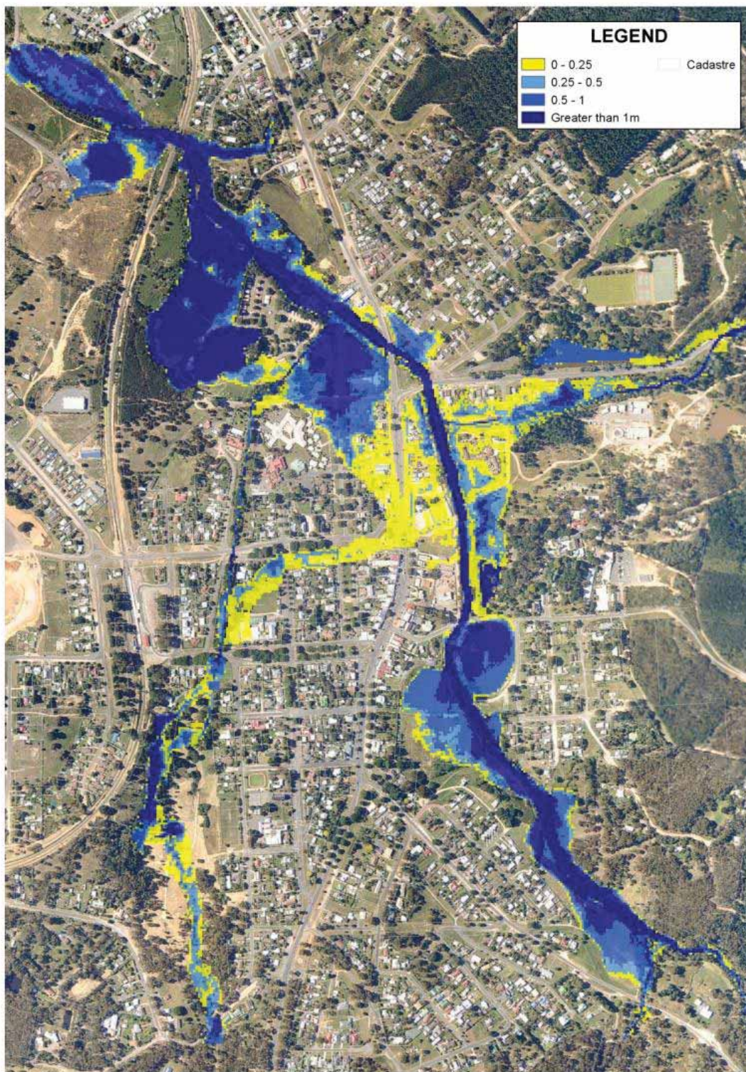
Figure 6-4 Proposed structural mitigation option 2 – 100 year ARI extent
