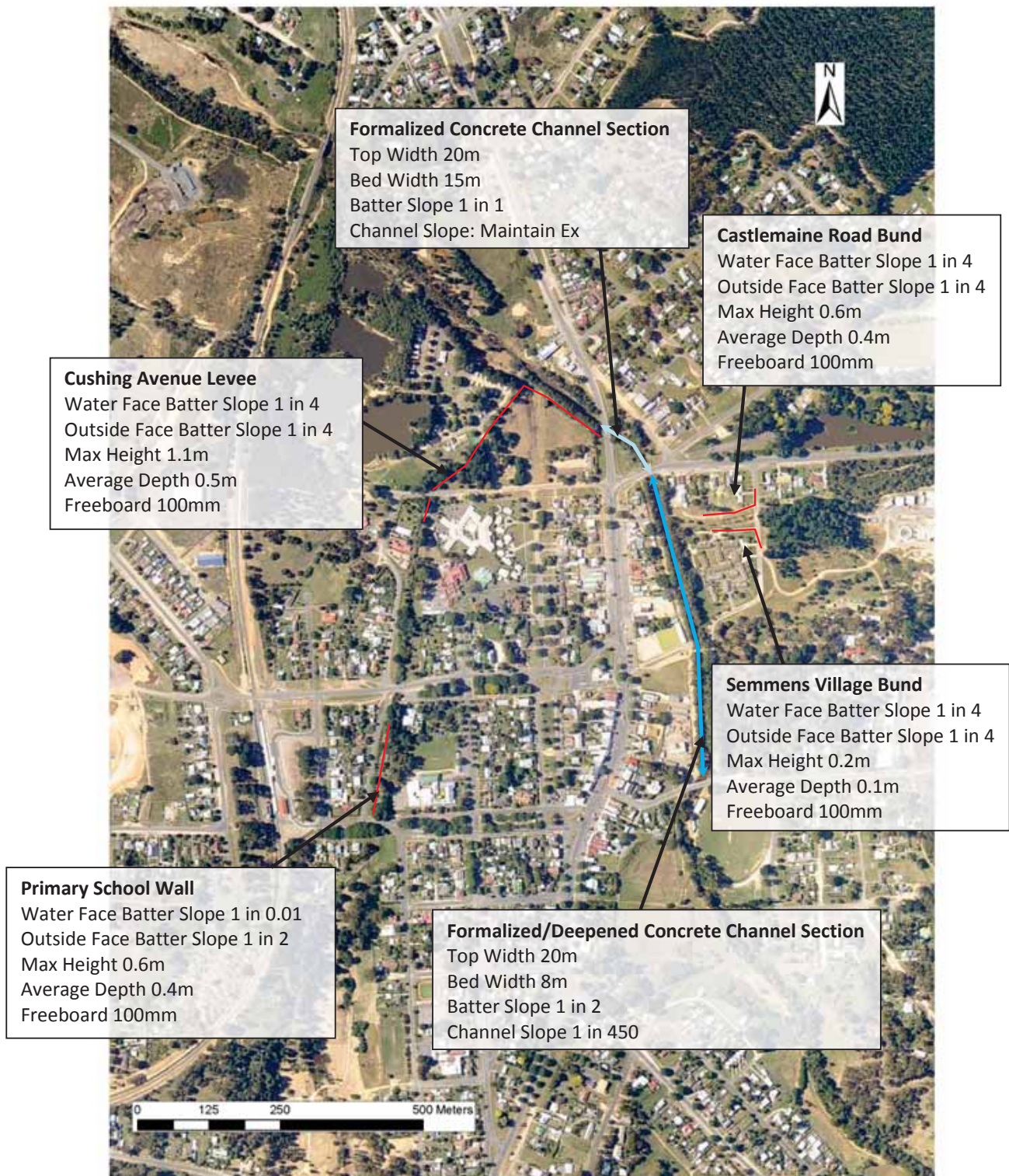
Figure 6-7 Proposed structural mitigation option 4
