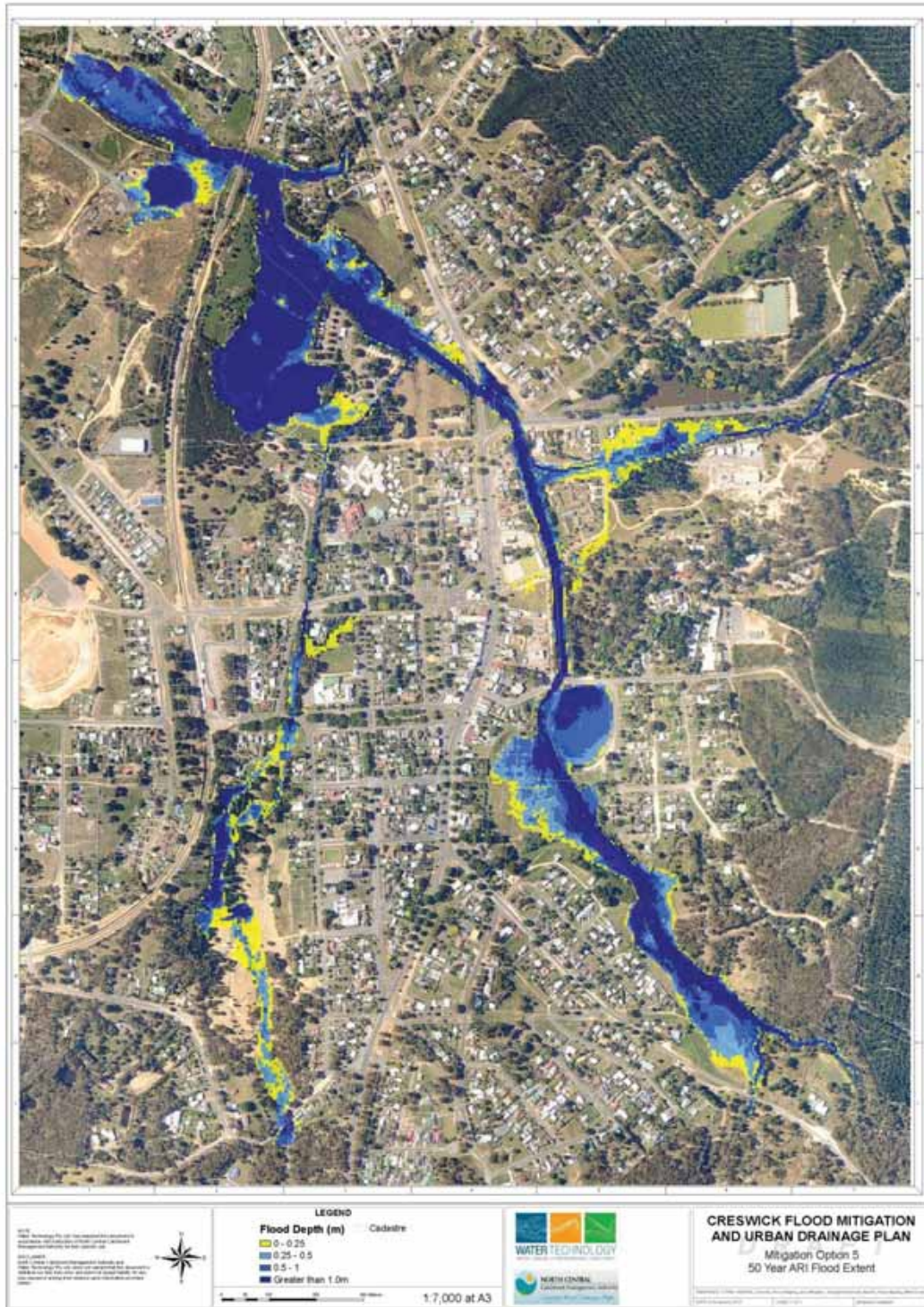
Figure E-3 50 Year ARI Flood Event
