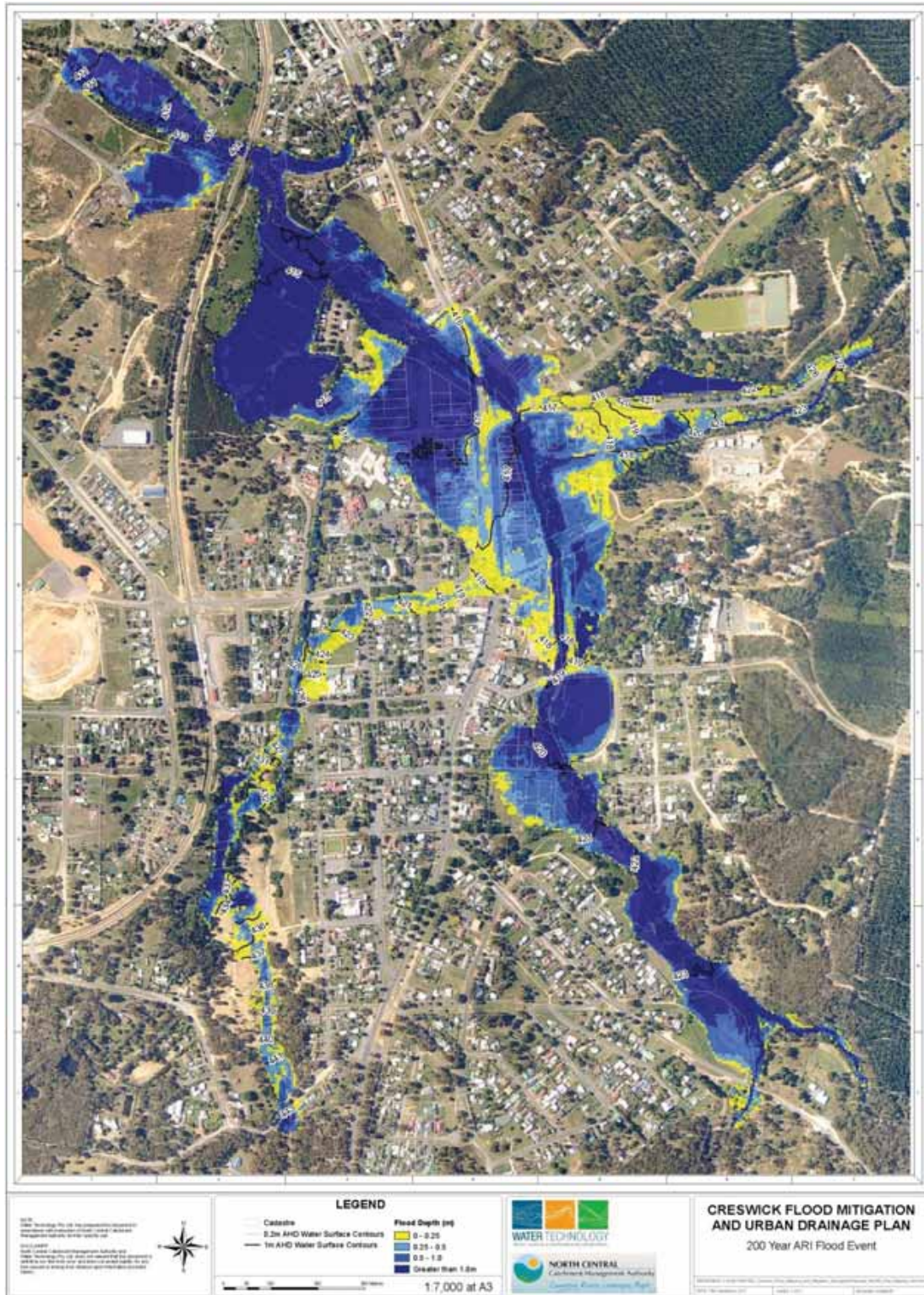
Figure C-9-6 200 Year ARI Flood Event
