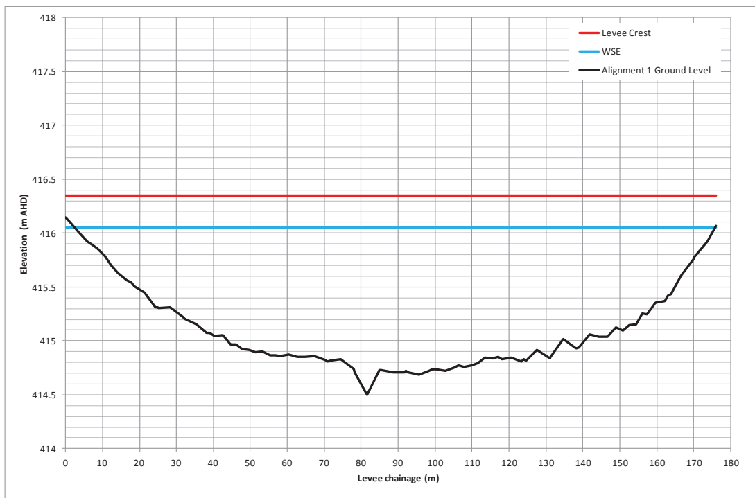
Figure D-9 North Parade Levee - Long Section Plot
