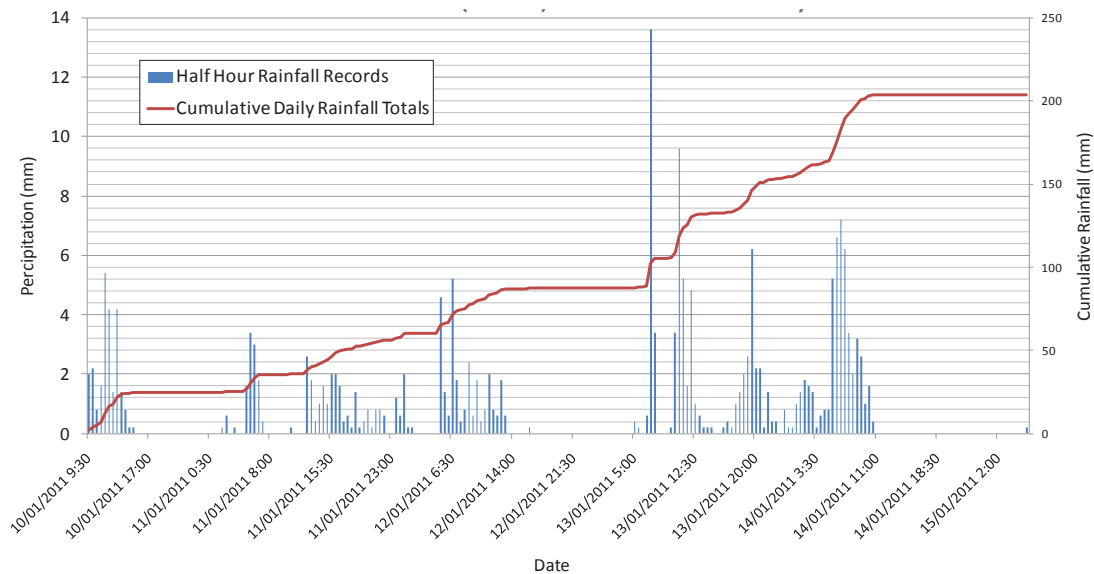
Figure 4-9 Ballarat Aerodrome (089002) pluviograph – January 2011
