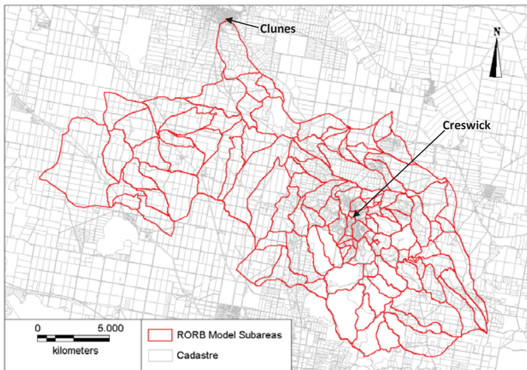
Figure 4-1 RORB model sub-area delineation
