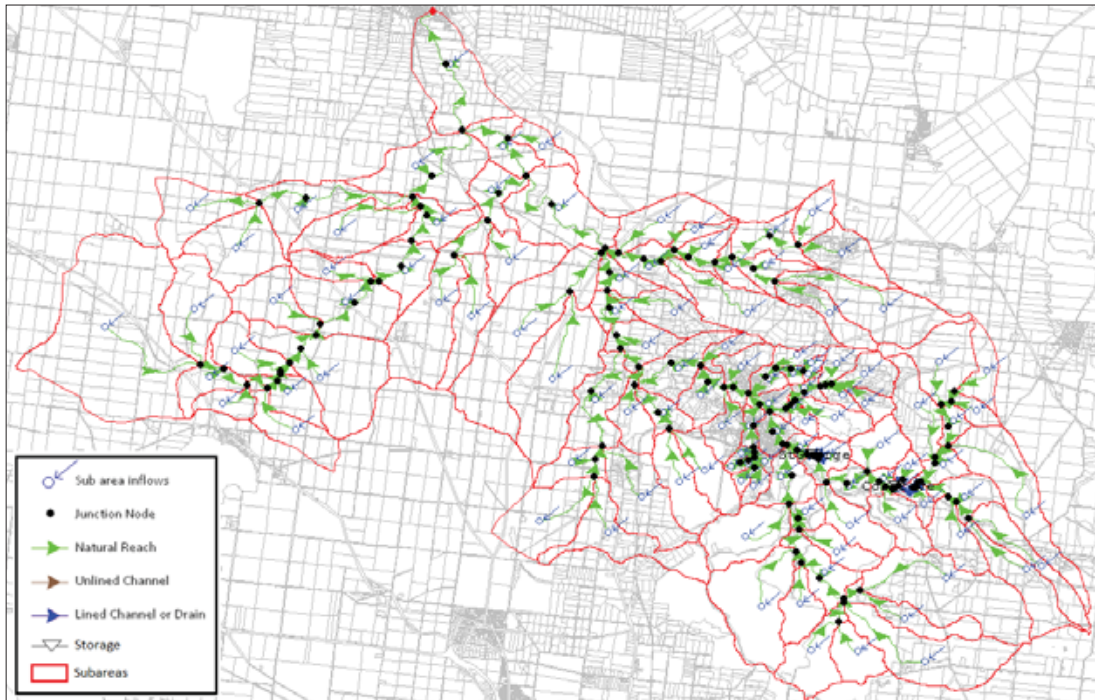
Figure 4-2 Graphical representation of the RORB model
