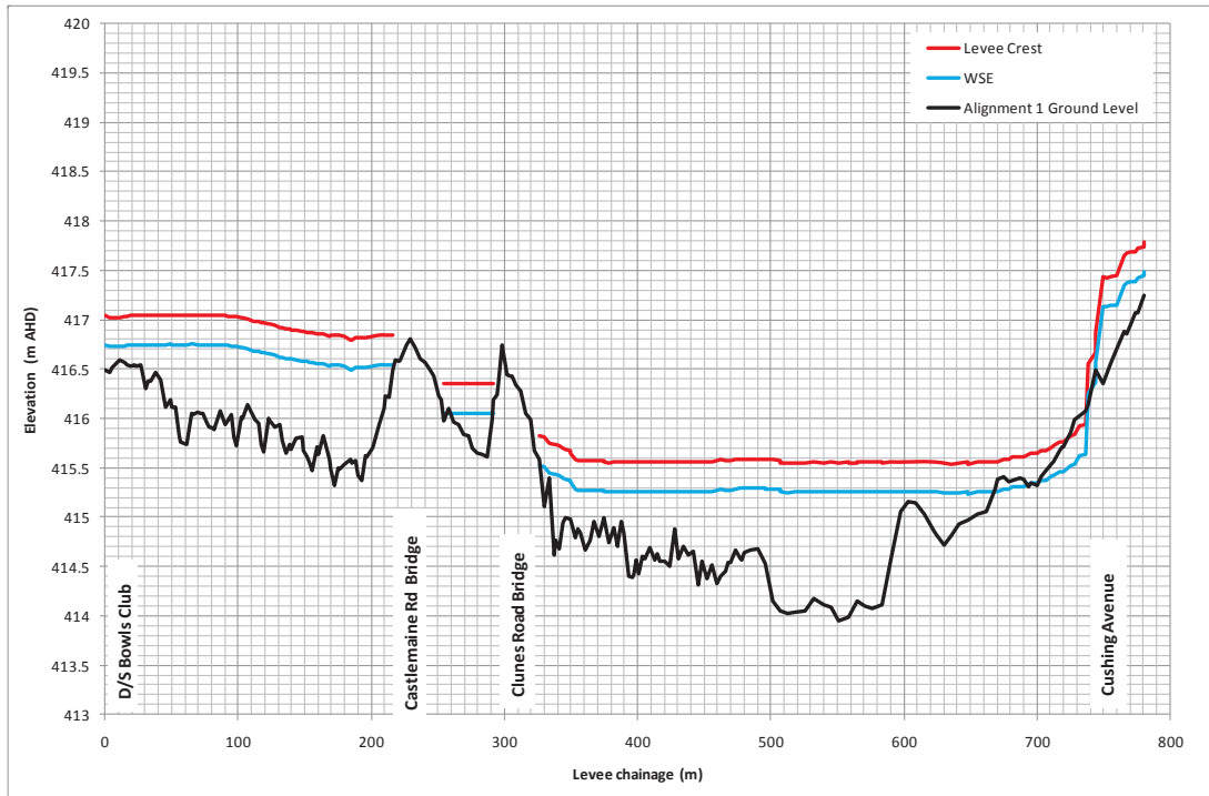
Figure D-1 Creswick Creek Levee - Long Section Plot
