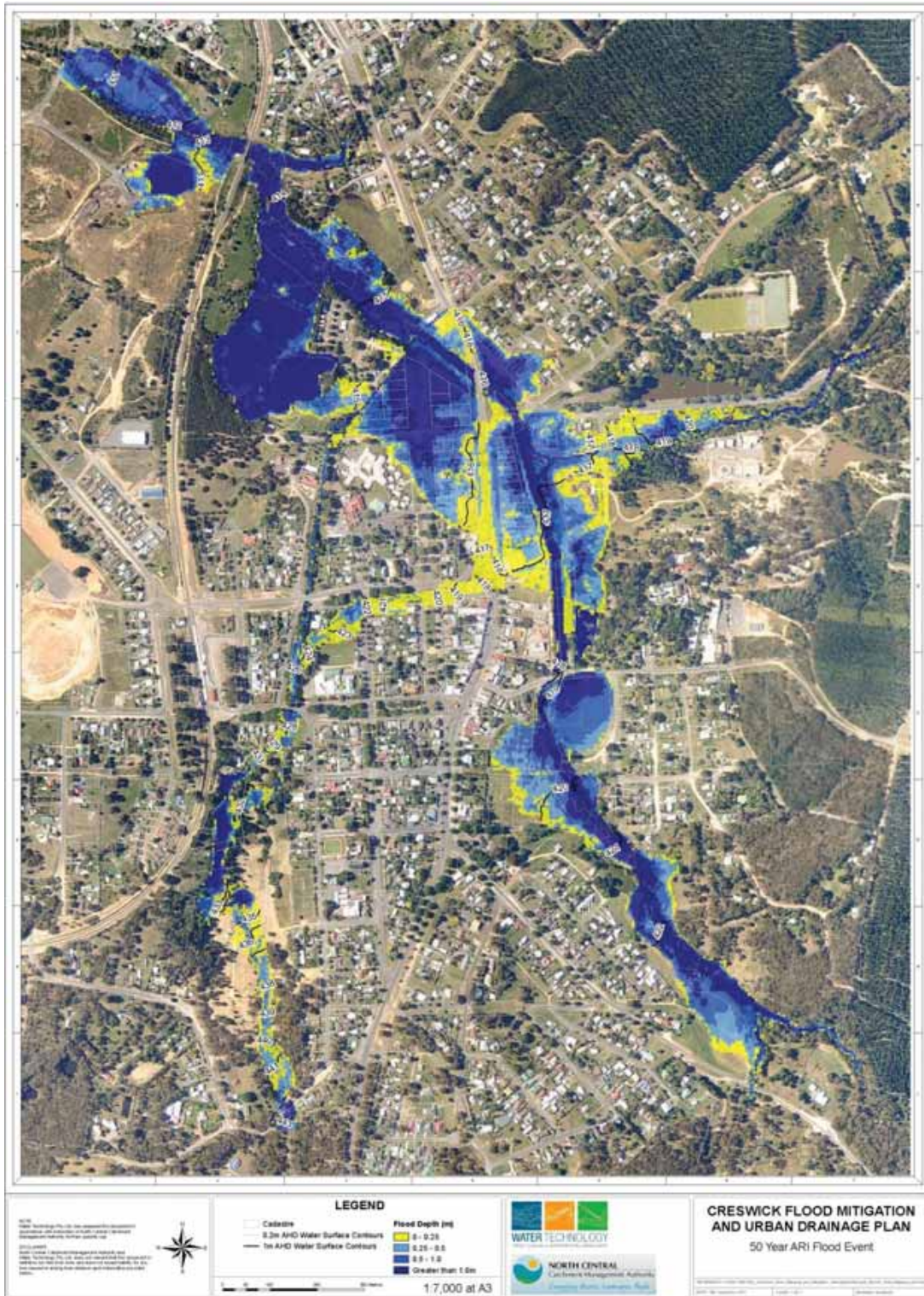
Figure C-9-4 50 Year ARI Flood Event
