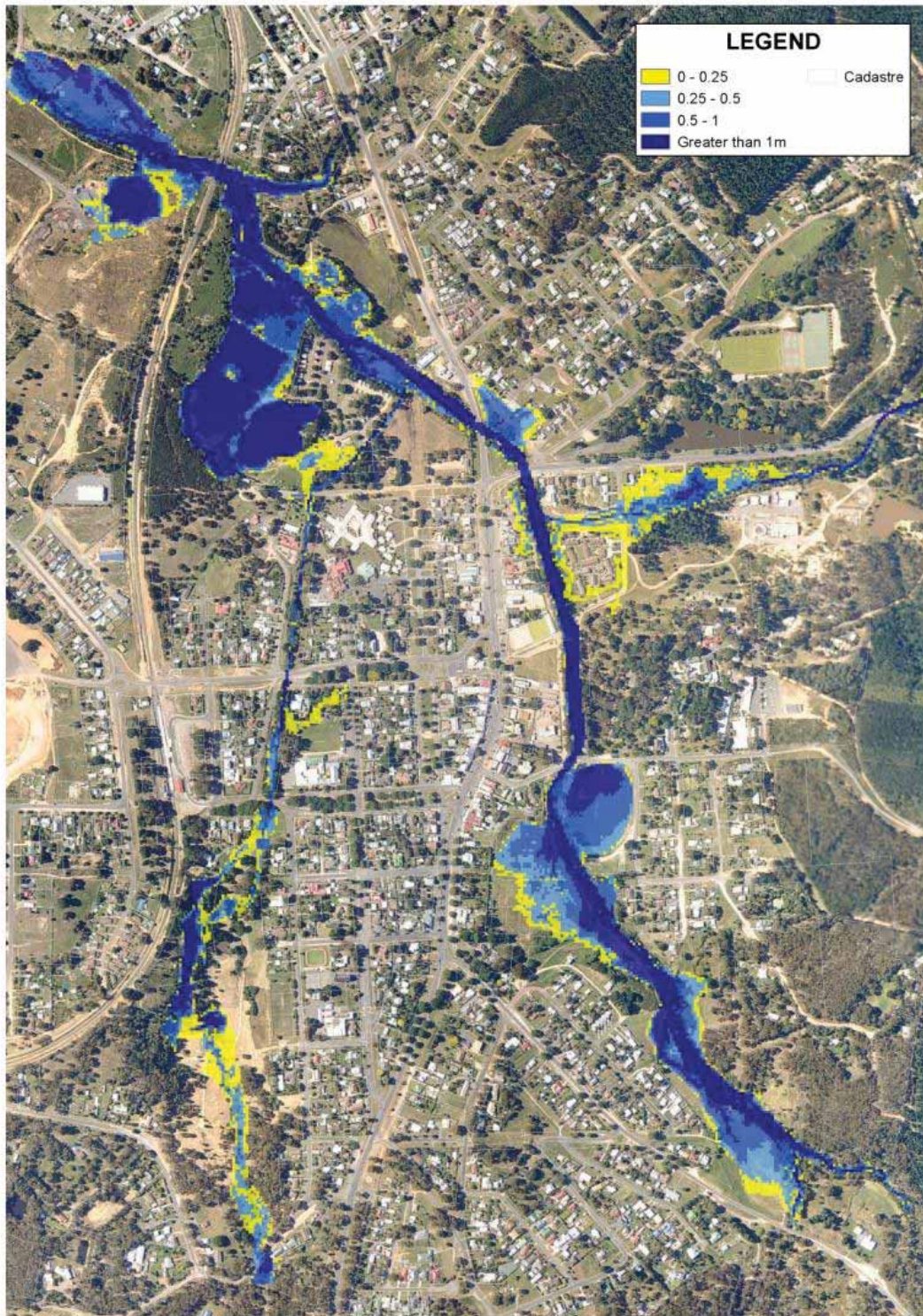
Figure 6-6 Proposed structural mitigation option 3 – 50 year ARI extent
