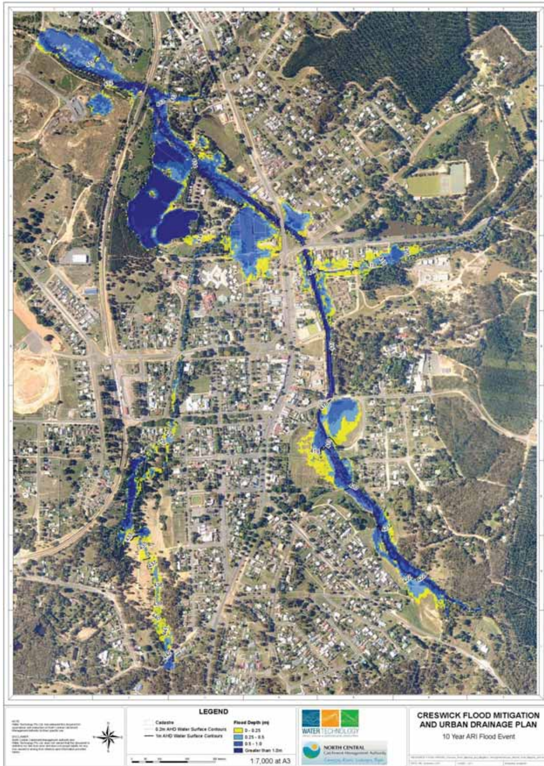
Figure C-9-2 10 Year ARI Flood Event
