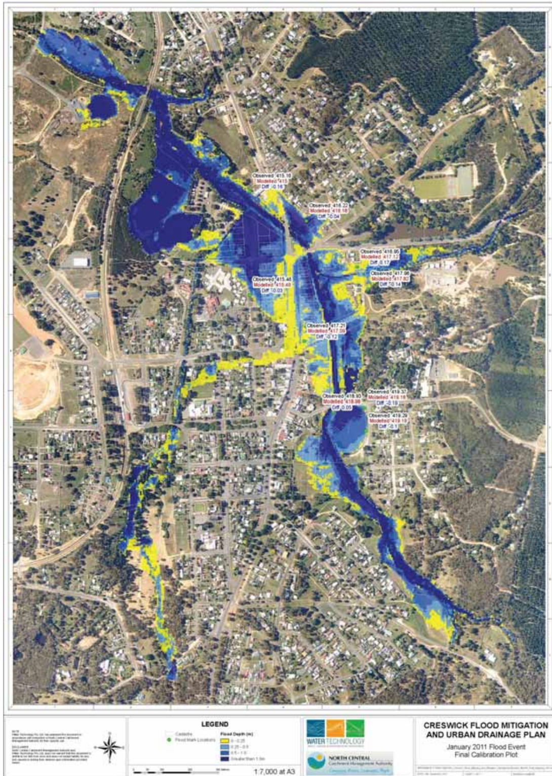
Figure 5-4 Hydraulic model calibration plot – January 2011
