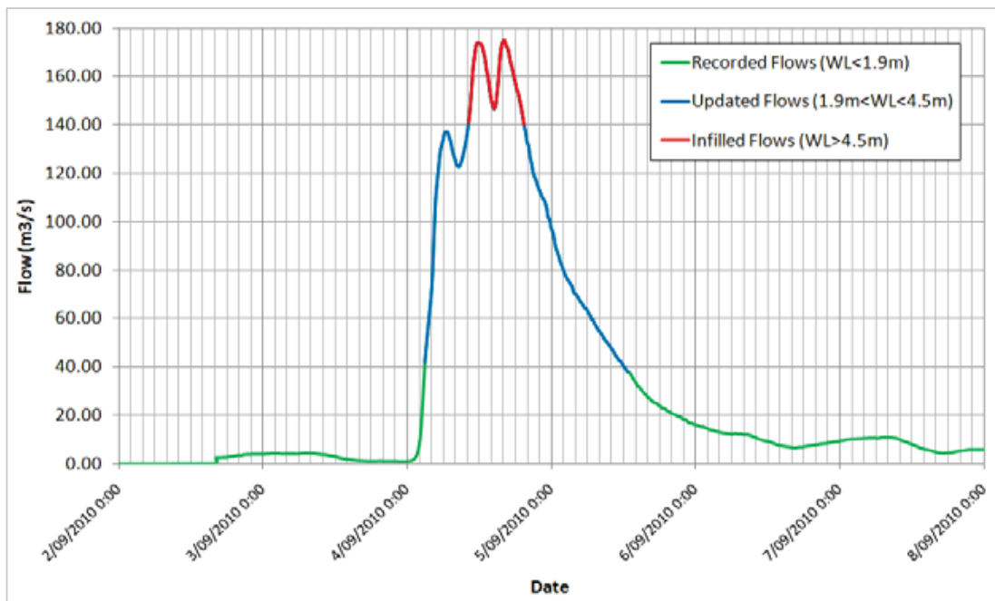
Figure 4-6 Creswick Creek @ Clunes flow hydrograph – September 2010
