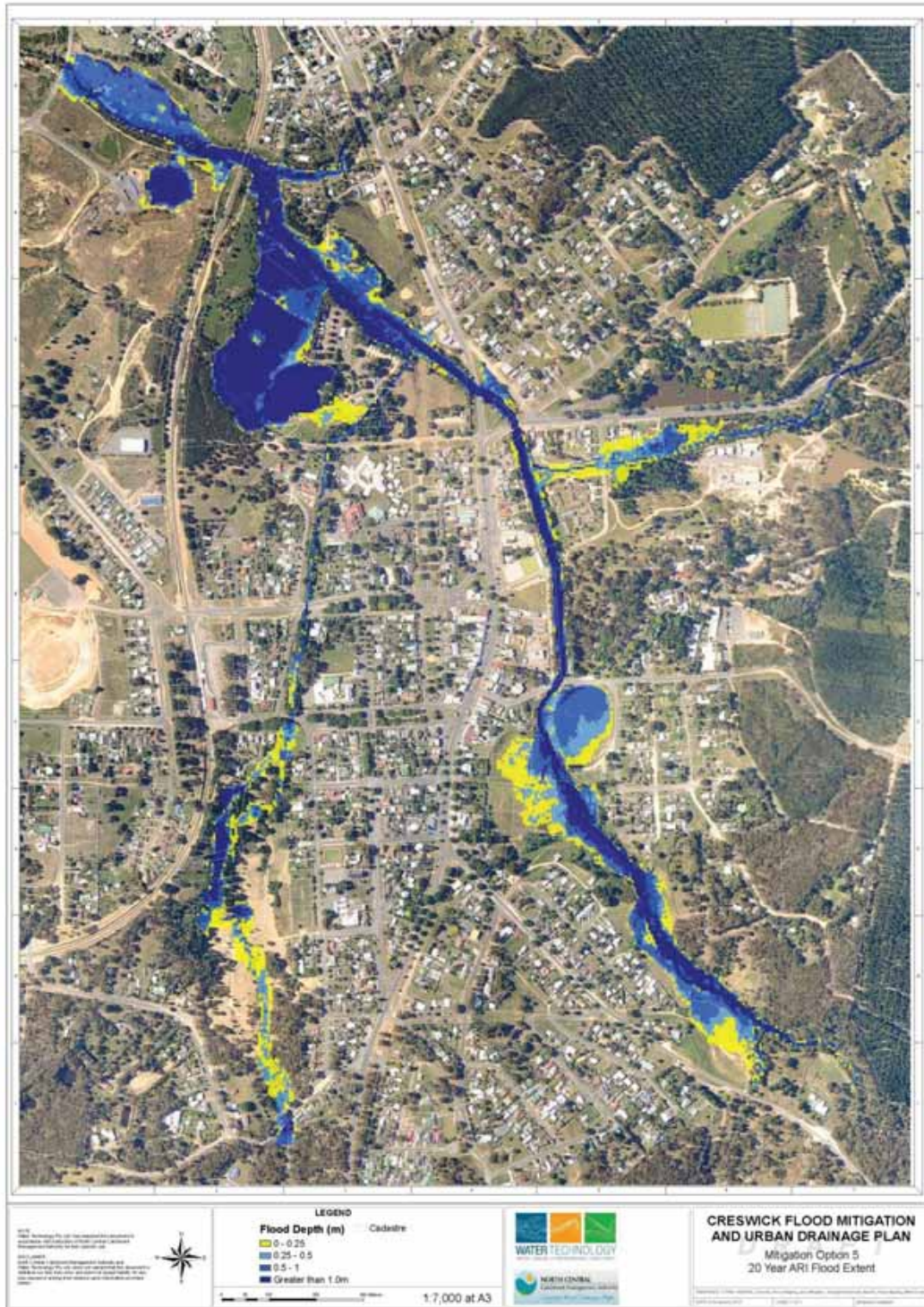
Figure E-2 20 Year ARI Flood Event
