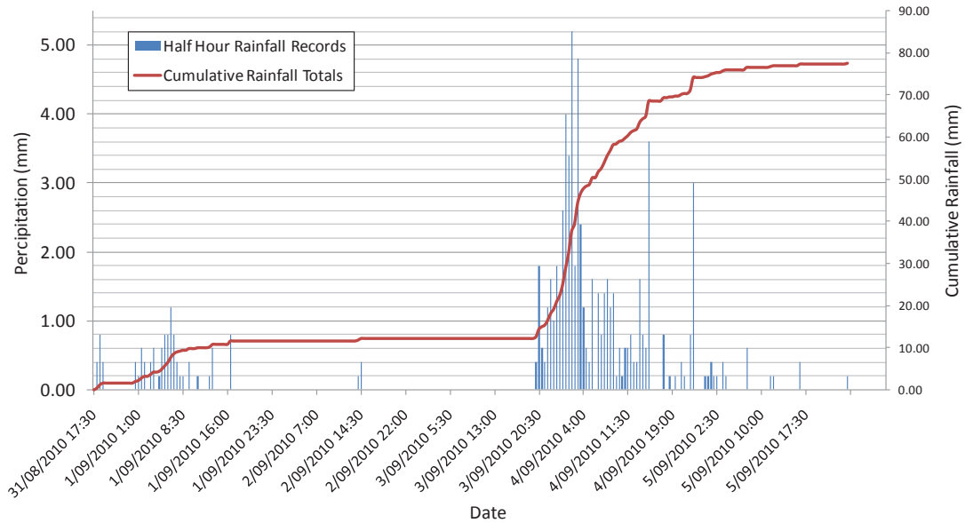
Figure 4-8 Ballarat Aerodrome (089002) pluviograph – September 2010
