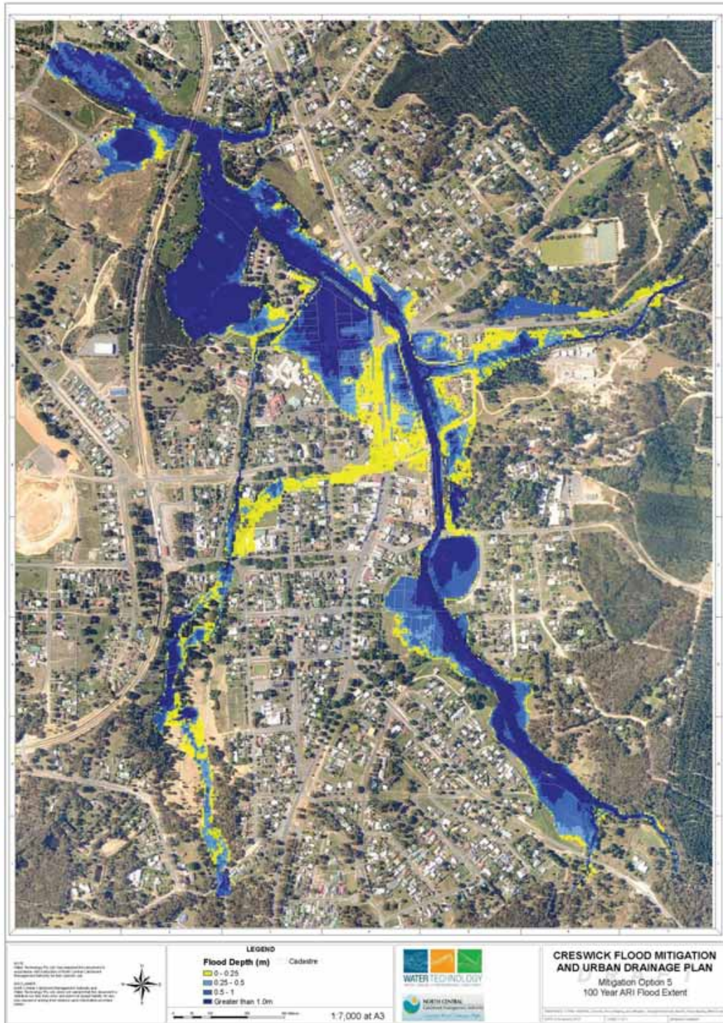
Figure E-4 100 Year ARI Flood Event
