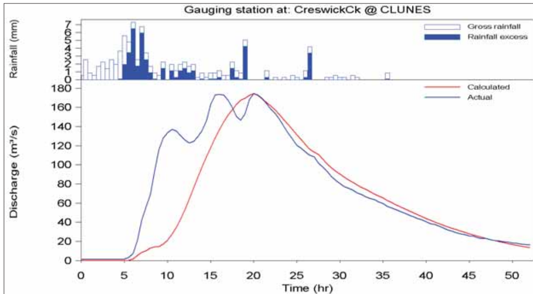
Figure 4-10 RORB model calibration hydrograph – September 2010
