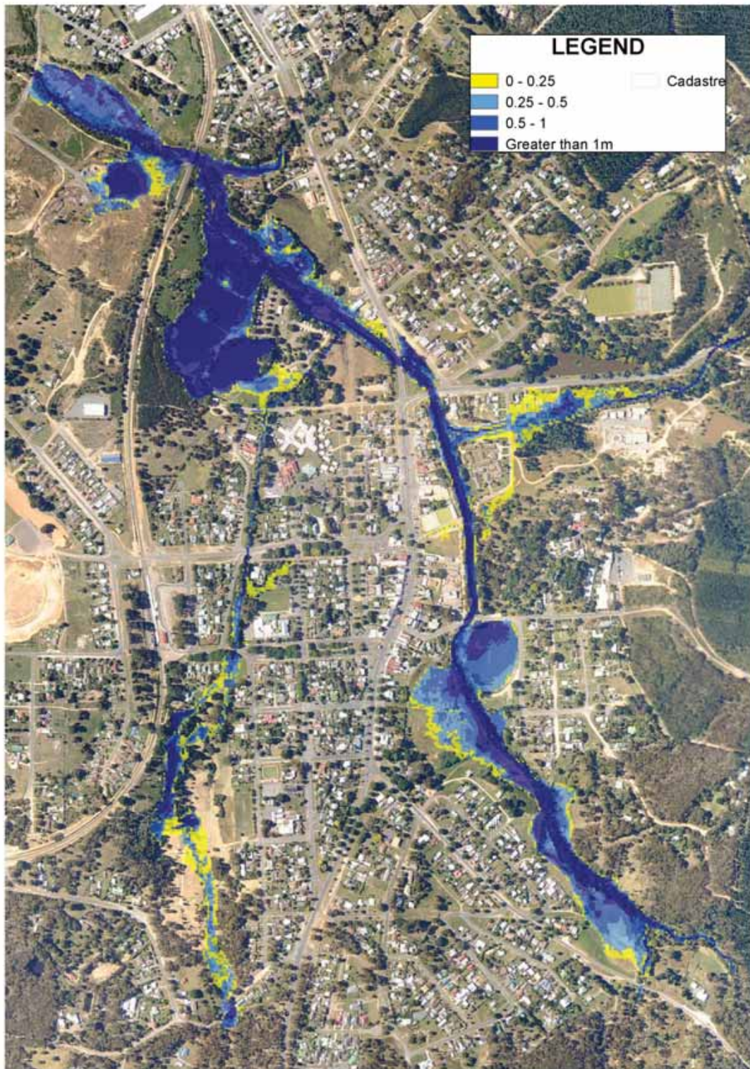
Figure 6-11 Proposed structural mitigation option 5 – 50 year ARI extent
