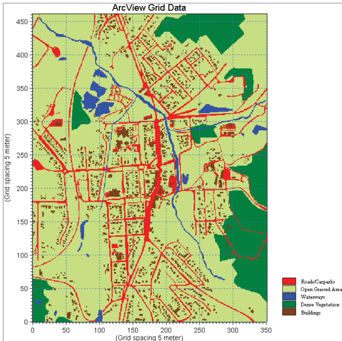
Figure 5-1 2D hydraulic model roughness grid
