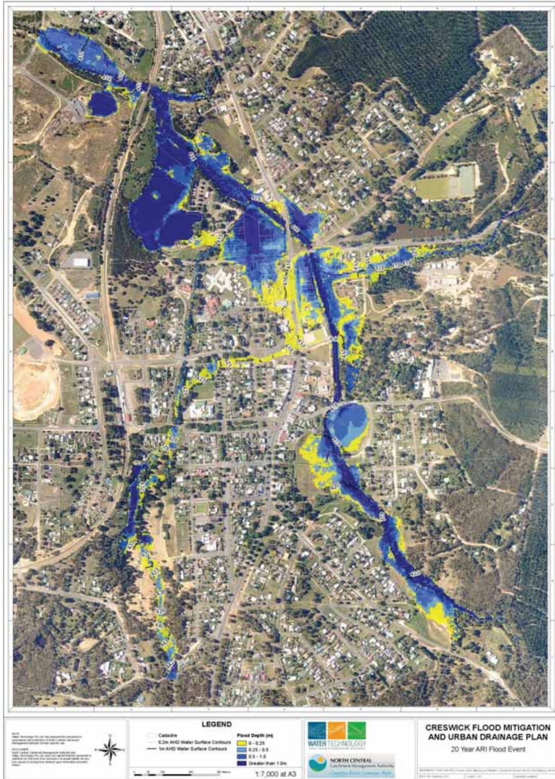
Figure C-9-3 20 Year ARI Flood Event
