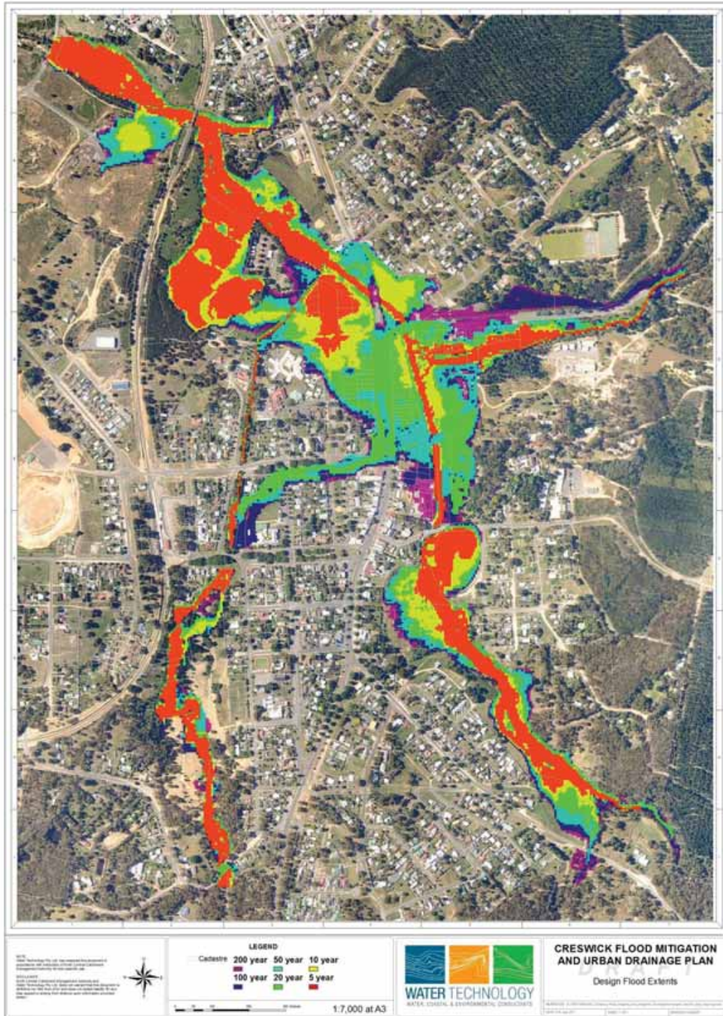
Figure 5-5 Hydraulic modelling design flood extents
