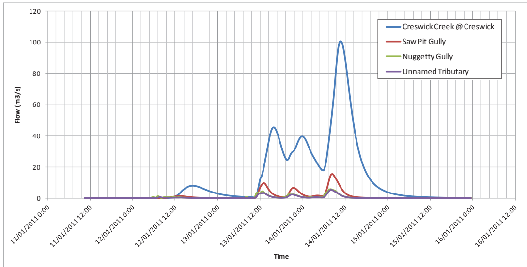
Figure 4-13 Flood hydrographs in Creswick – January 2011
