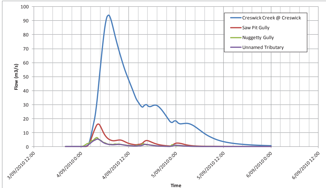
Figure 4-12 Flood hydrographs in Creswick – September 2010
