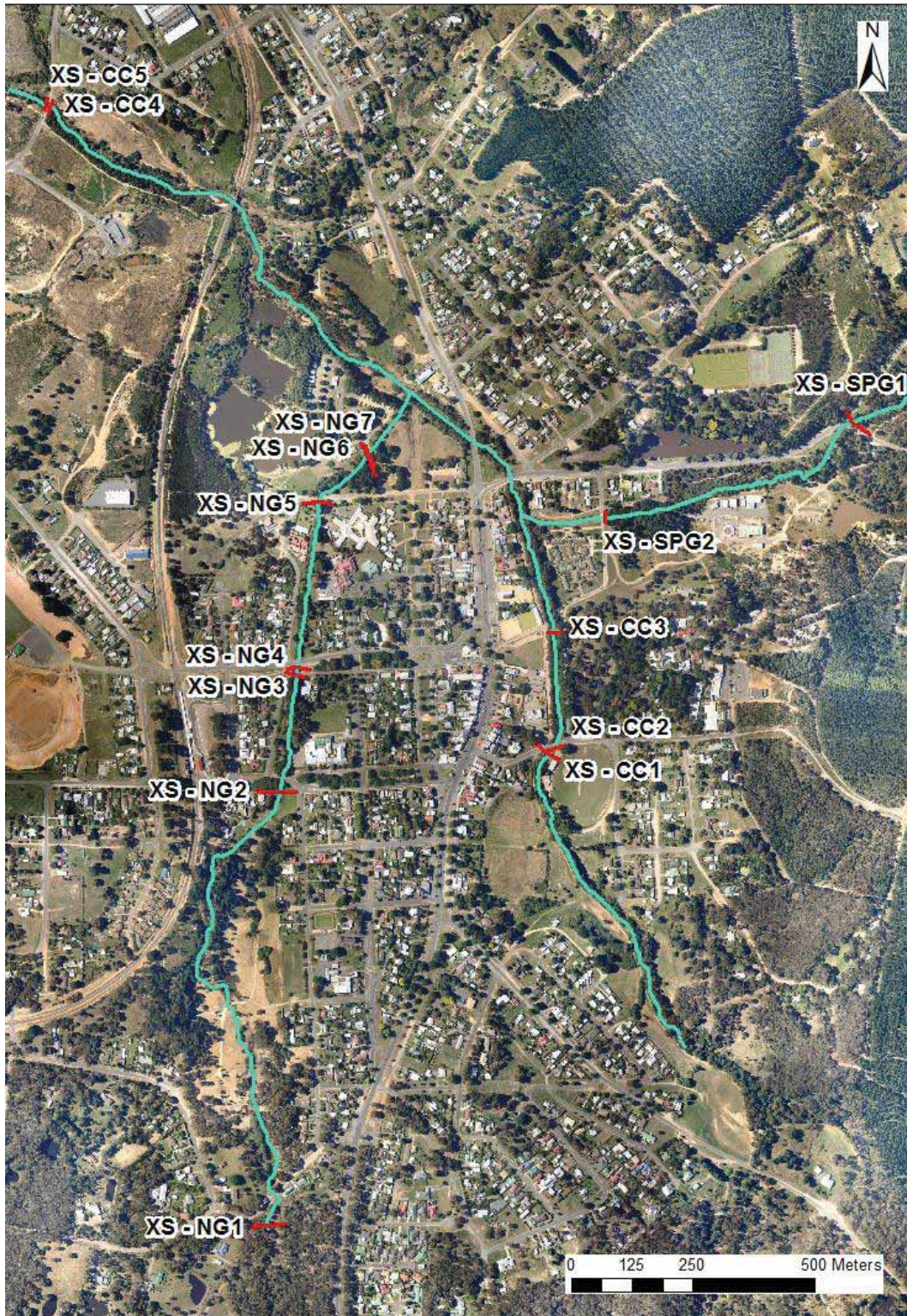
Figure B 2 Location of Surveyed Cross Sections
