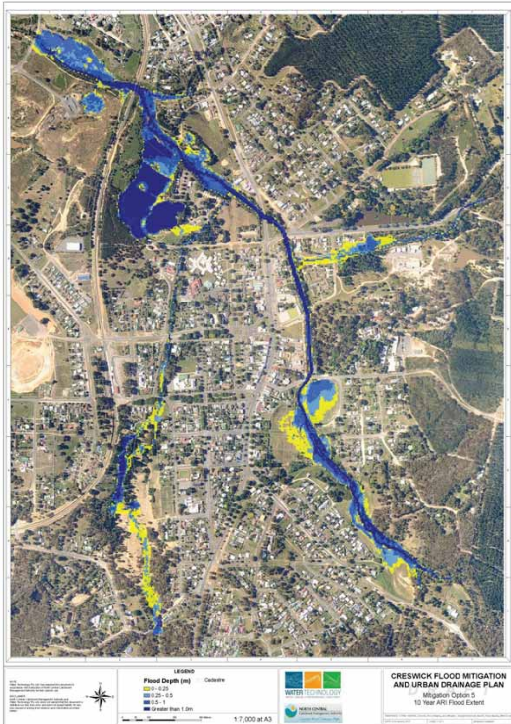
Figure E-1 10 Year ARI Flood Event
