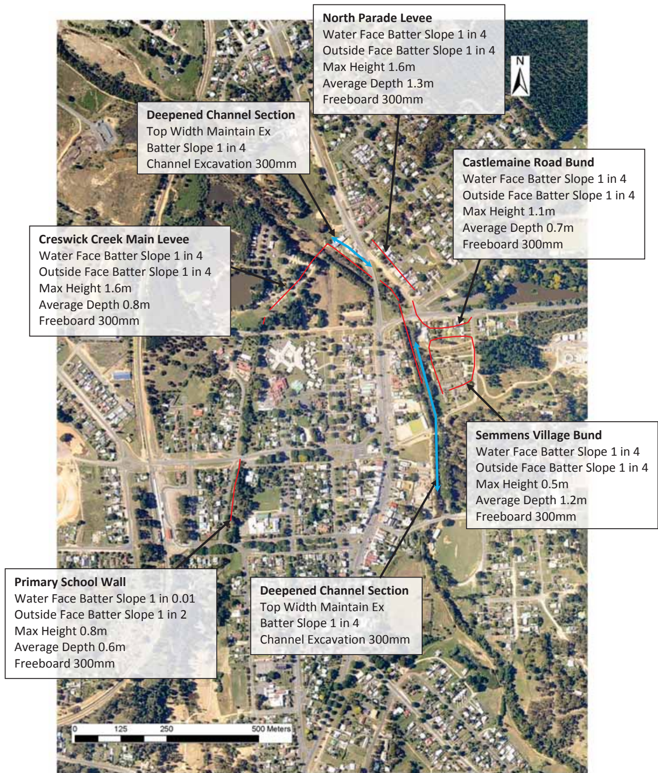
Figure 6-10 Proposed structural mitigation option 5
