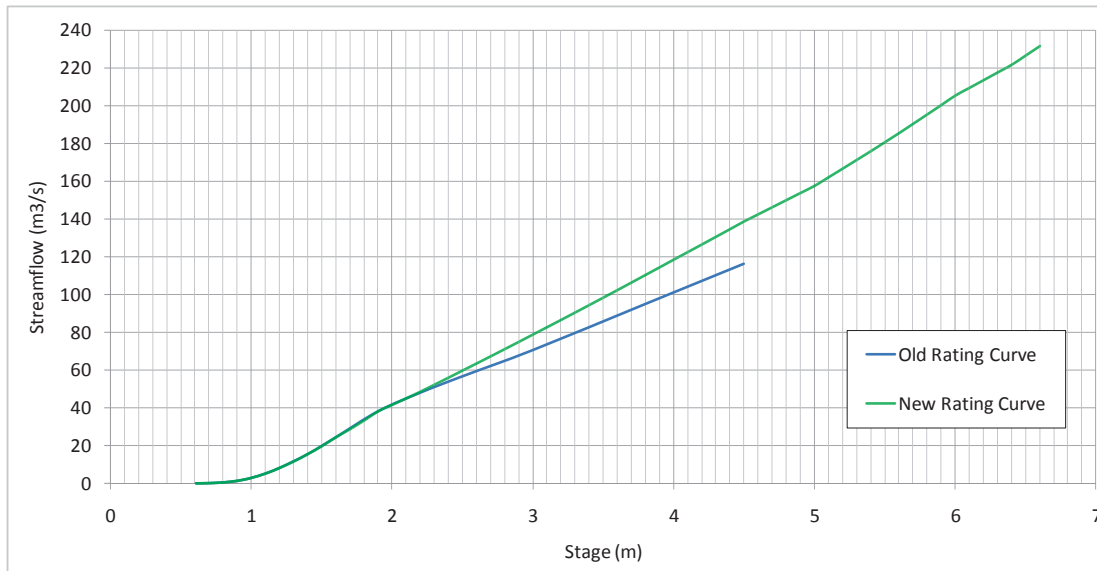
Figure 4-5 Creswick Creek @ Clunes gauge rating curve
