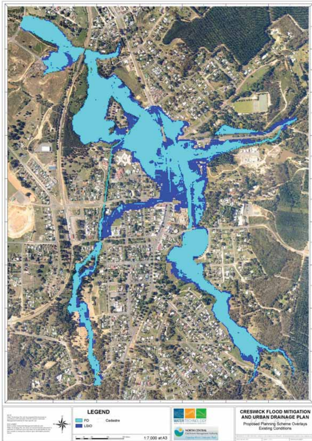
Figure 6-14 Draft LSIO and FO maps for existing conditions
