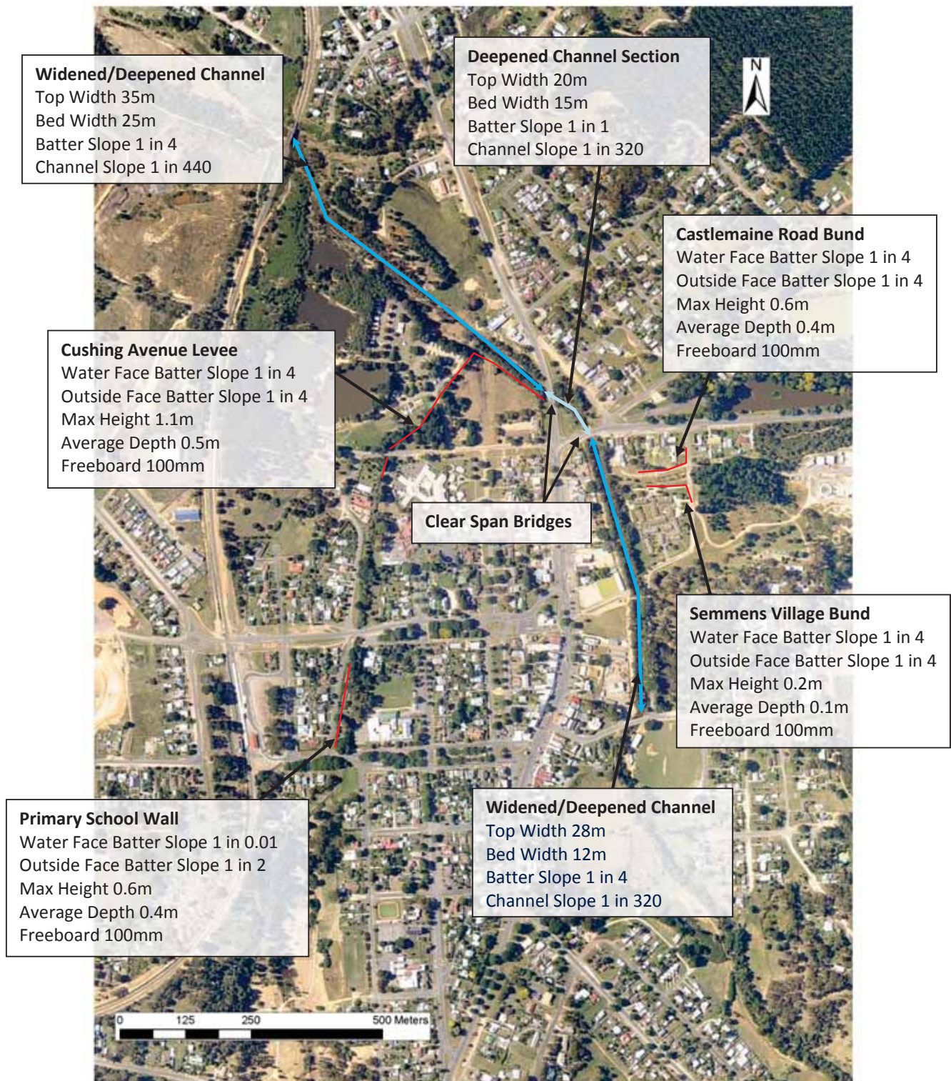
Figure 6-5 Proposed structural mitigation option 3
