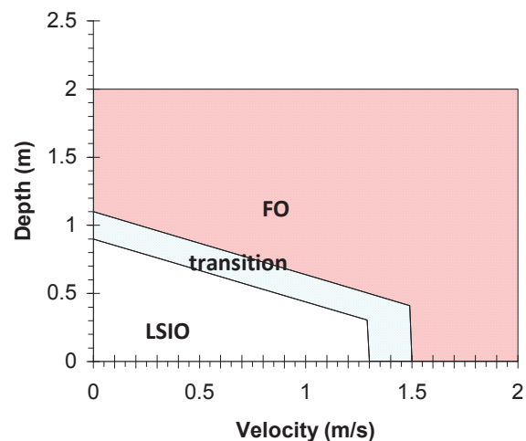
Figure 6-12 Flood hazard delineation of FO
