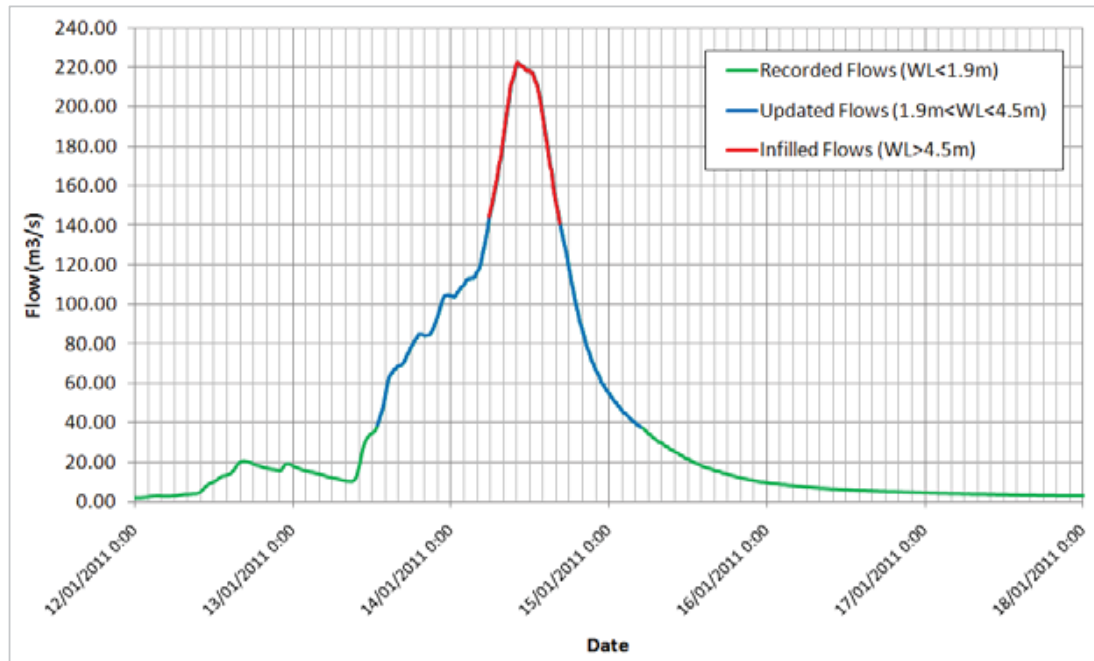
Figure 4-7 Creswick Creek @ Clunes flow hydrograph – January 2011
