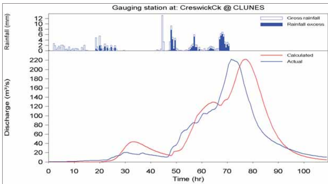
Figure 4-11 RORB model calibration hydrograph – January 2011
