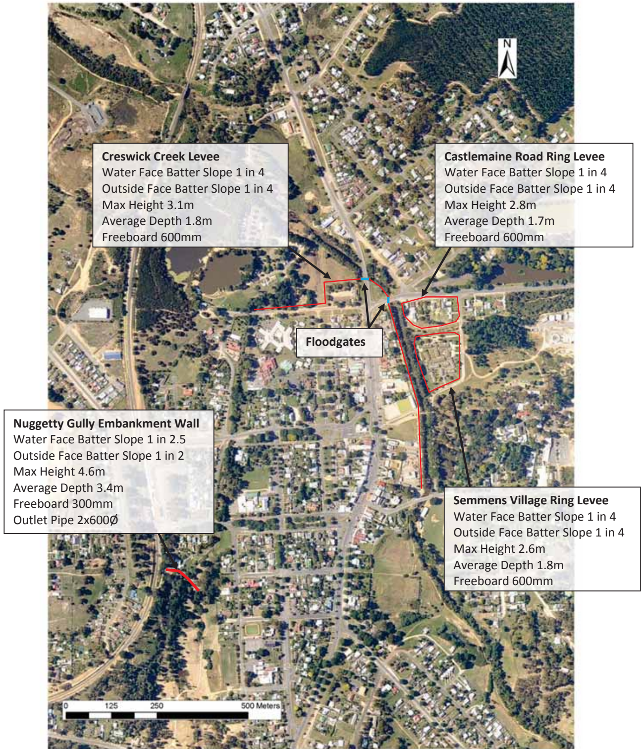
Figure 6-1 Proposed structural mitigation option 1
