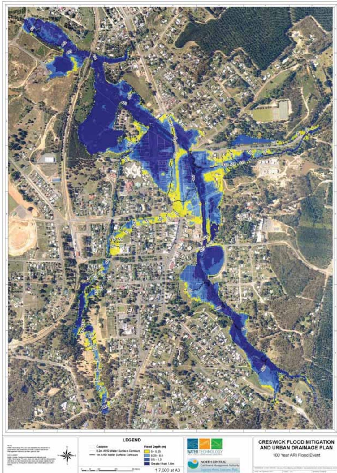
Figure C-9-5 100 Year ARI Flood Event
